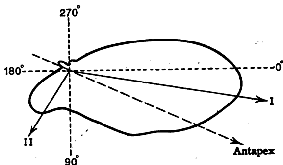
II. Region II. ; centre, R.A. 0 h , Dec. +50°.
